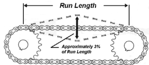
DETERMINING CHAIN SLACK
