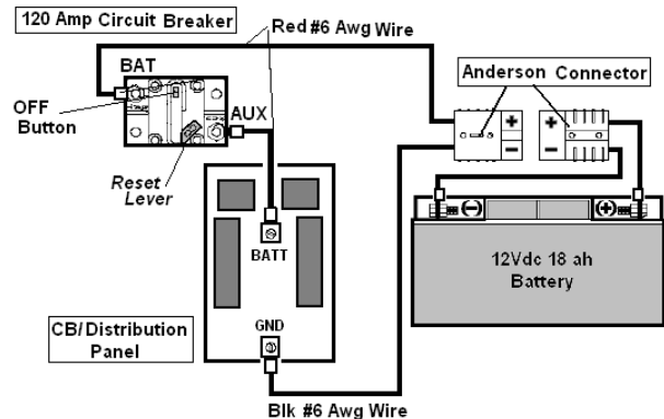
2005 Main Power Connections
