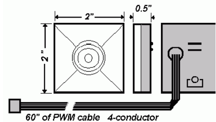
Hi-Intensity LED Clusters
